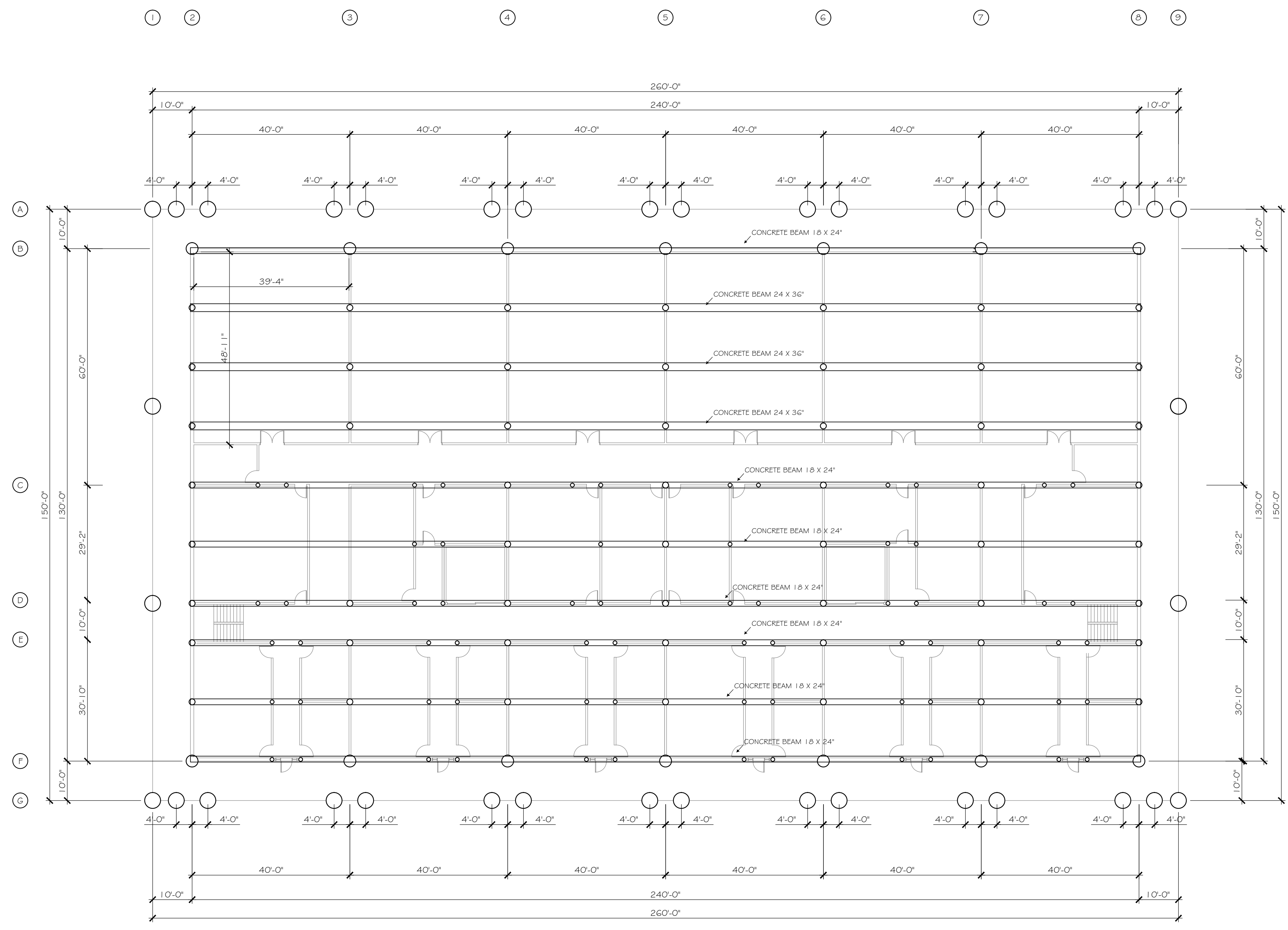
ROOF BEAM STRUCTURE SCALE: 1/16" = 1'-0" REVISED - FEB 14, 2022
